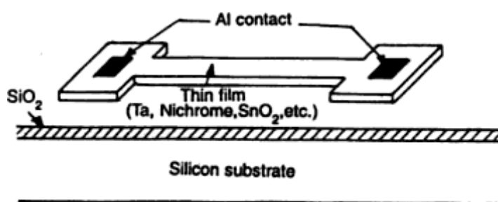
Fig. 1.23 (c) Cross-section of a thin film resistor
